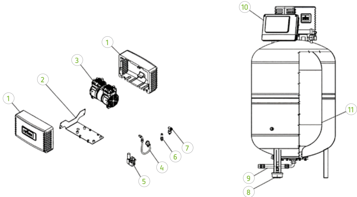
Reflexomat Silent Compact Smart
