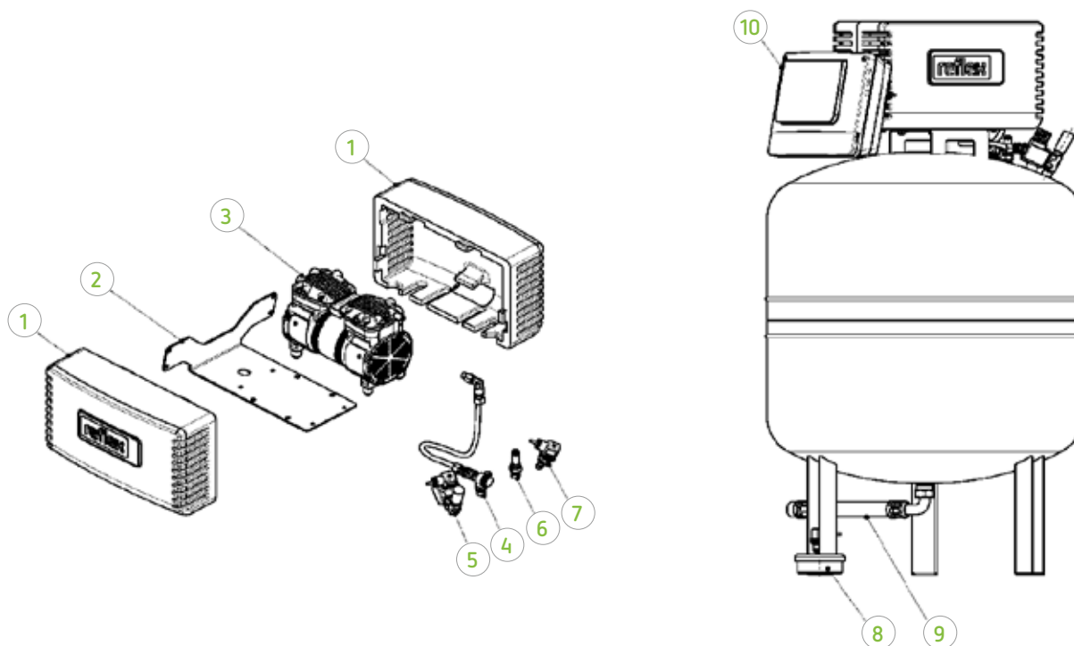
Reflexomat Silent Compact
