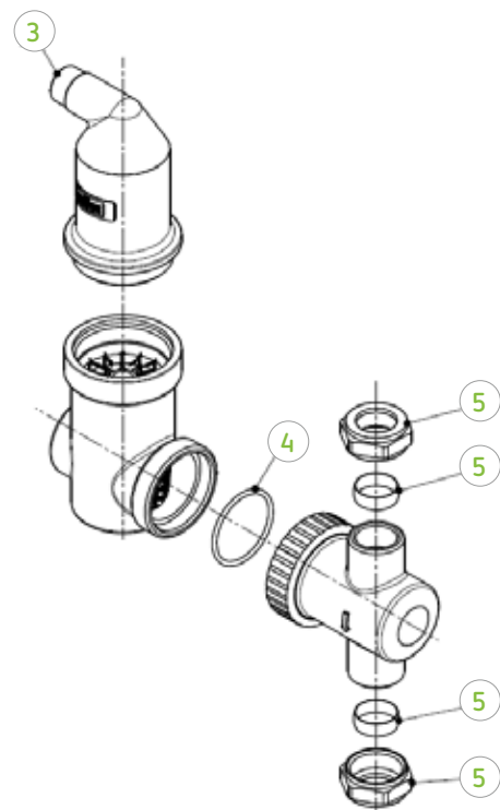
Exvoid Twist AT 22 M
