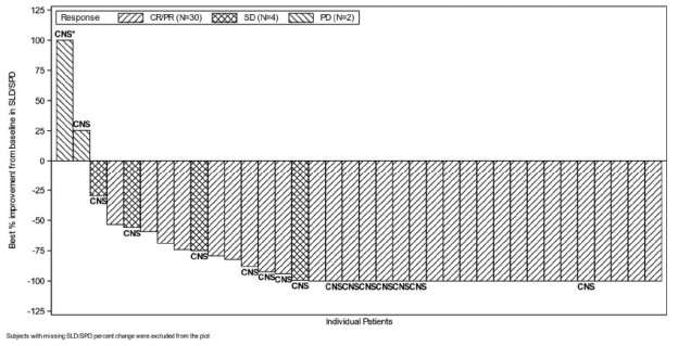
Figure 2: Best percentage change from baseline in tumor size (BICR assessment) in pediatric patients with NTRK -fusion positive solid tumors (primary CNS and non-CNS), shaded by response
