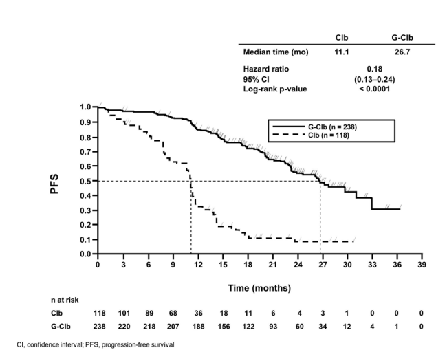
Figure 1 Kaplan-Meier curve of Investigator assessed progression-free survival from Stage 1
