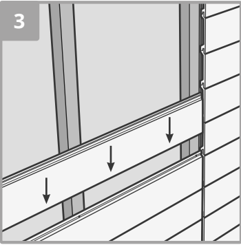
Repeat, making sure to shape boards around openings.
