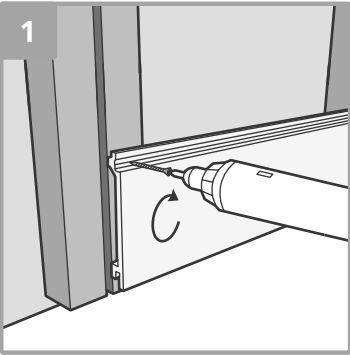
Pre-drill oversized holes and fix with screws to the substructure.
