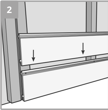
Clip the second board to the groove of the first board.
