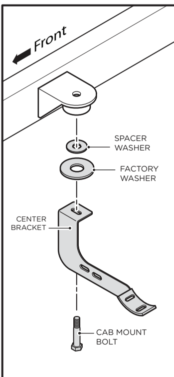
Center Bracket
