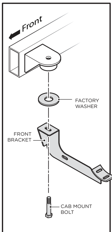
Front Bracket
