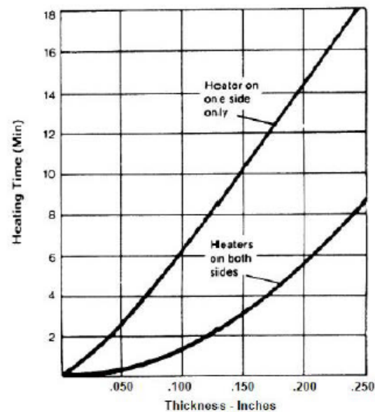
FIGURE 16 - Electric Infra-Red Radiant Heating
