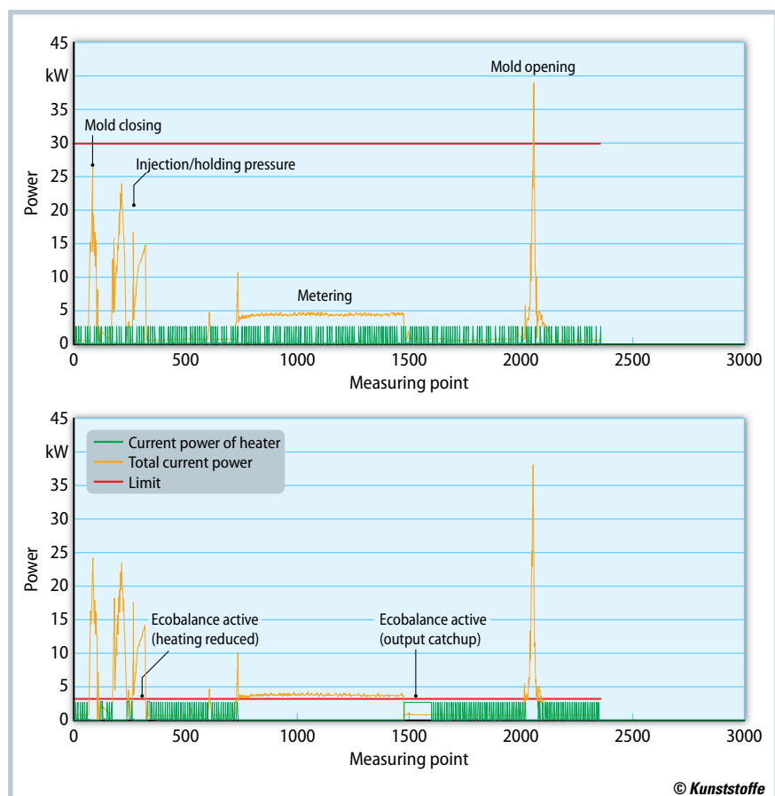
Fig. 4. The Engel e-victory 440/120 injection molding machine illustrates how ecobalance can be used to lower the energy limit from 30 kW (above) to 3 kW (below) (© Engel)
