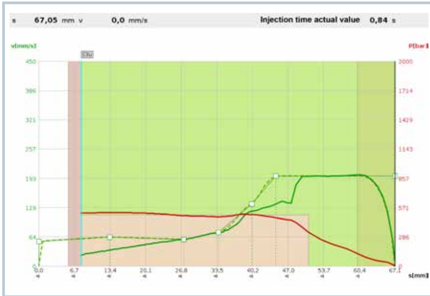
Fig. 3. The red area stands for the pressure control. It illustrates the holding pressure phase and possible intervention by the pressure limit controller (© Engel)
