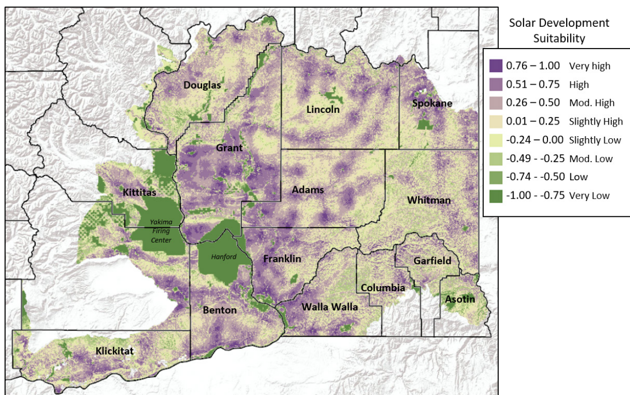
Figure 6. Final solar development suitability map results for the Washington Columbia Plateau.
