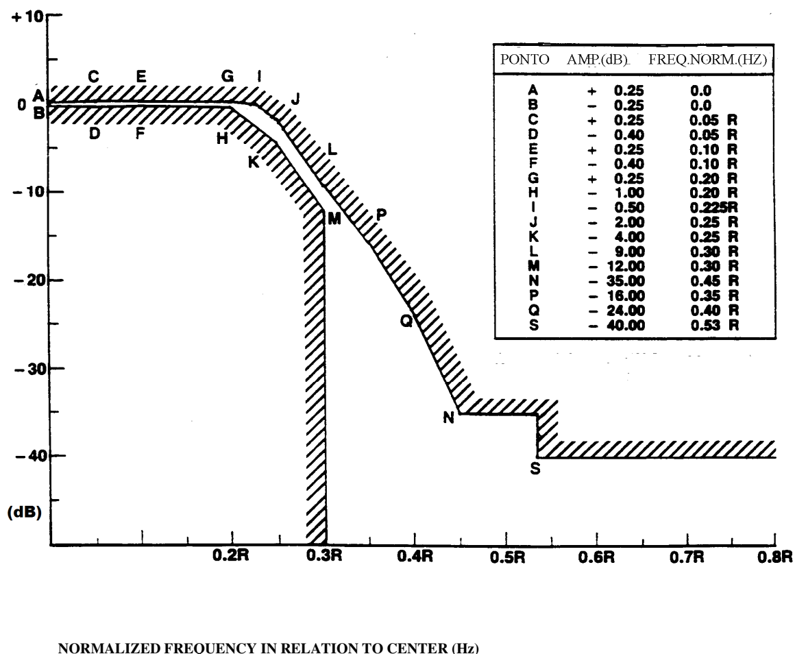
Figure 3 - Spectral Power Density Mask at Modulator Output
