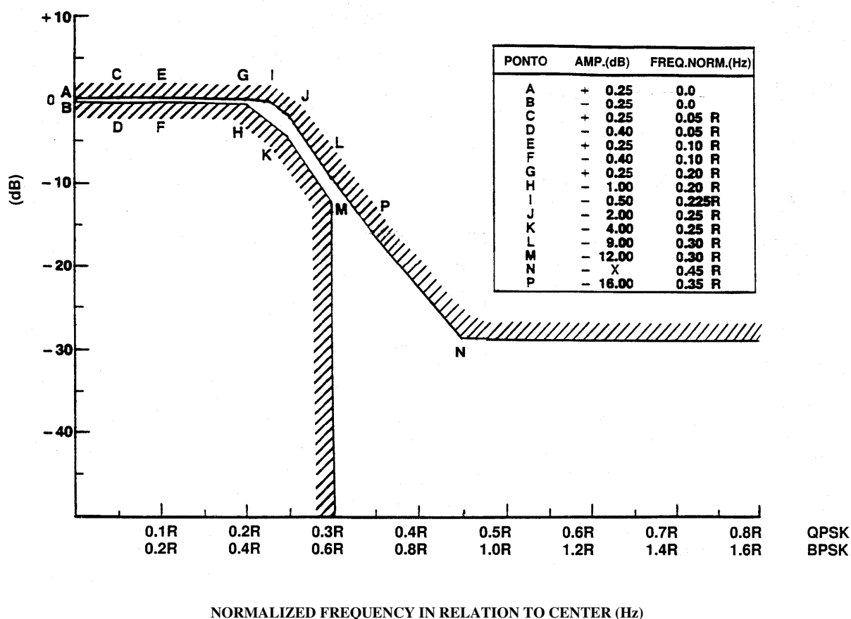
Figure 4 - Spectral Power Density Mask at Transmitter Output
